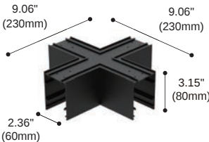
Article number: BNT-15 Type : X Type horizontal connector
